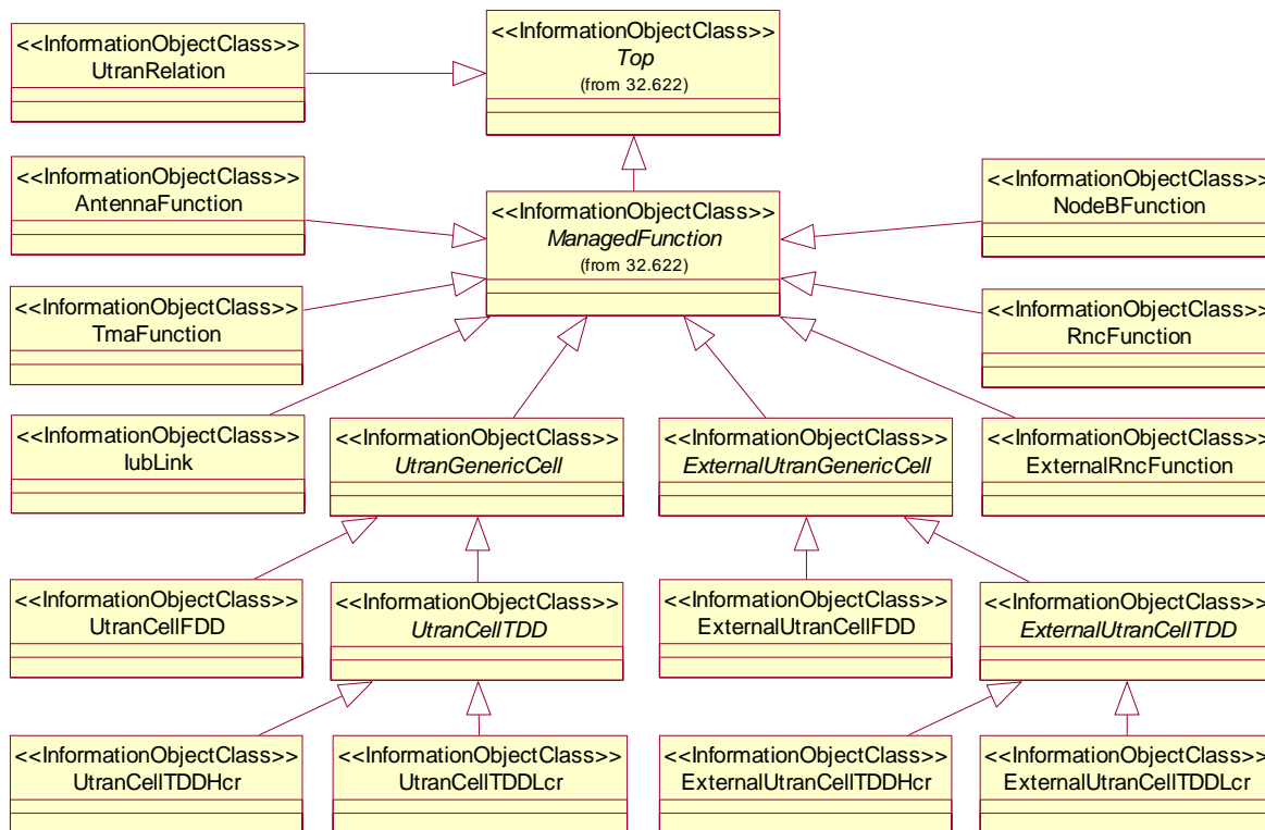
Figure 6.2.2.1: UTRAN NRM Inheritance Hierarchy
