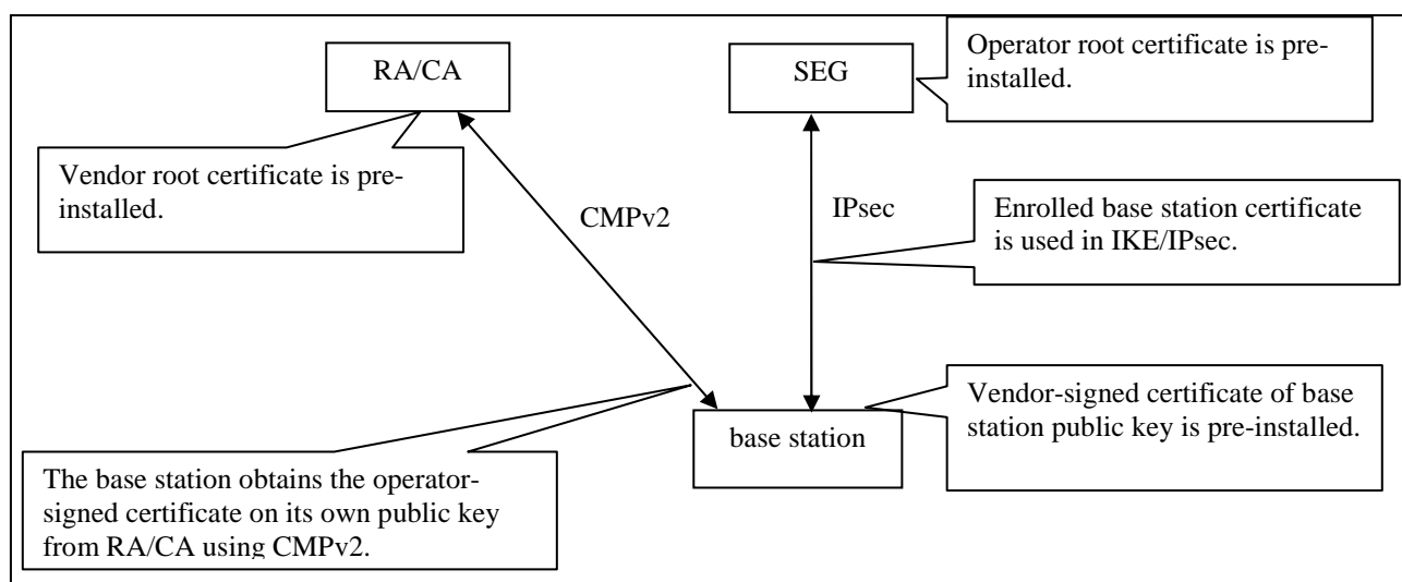
Figure 7: Overview of the security architecture
