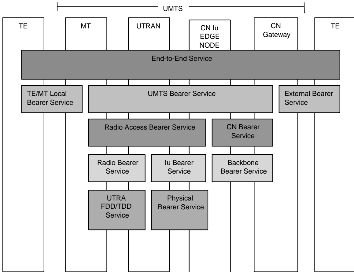
Figure 6.10.1.1: UMS QoS Architecture
