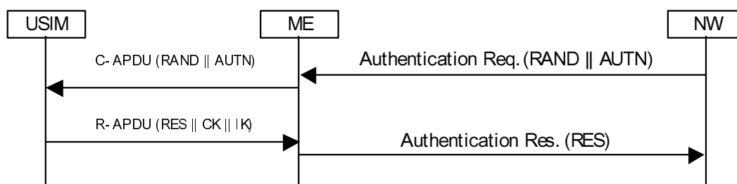
Figure 8.1.2.3.1: Network accepted by UE
