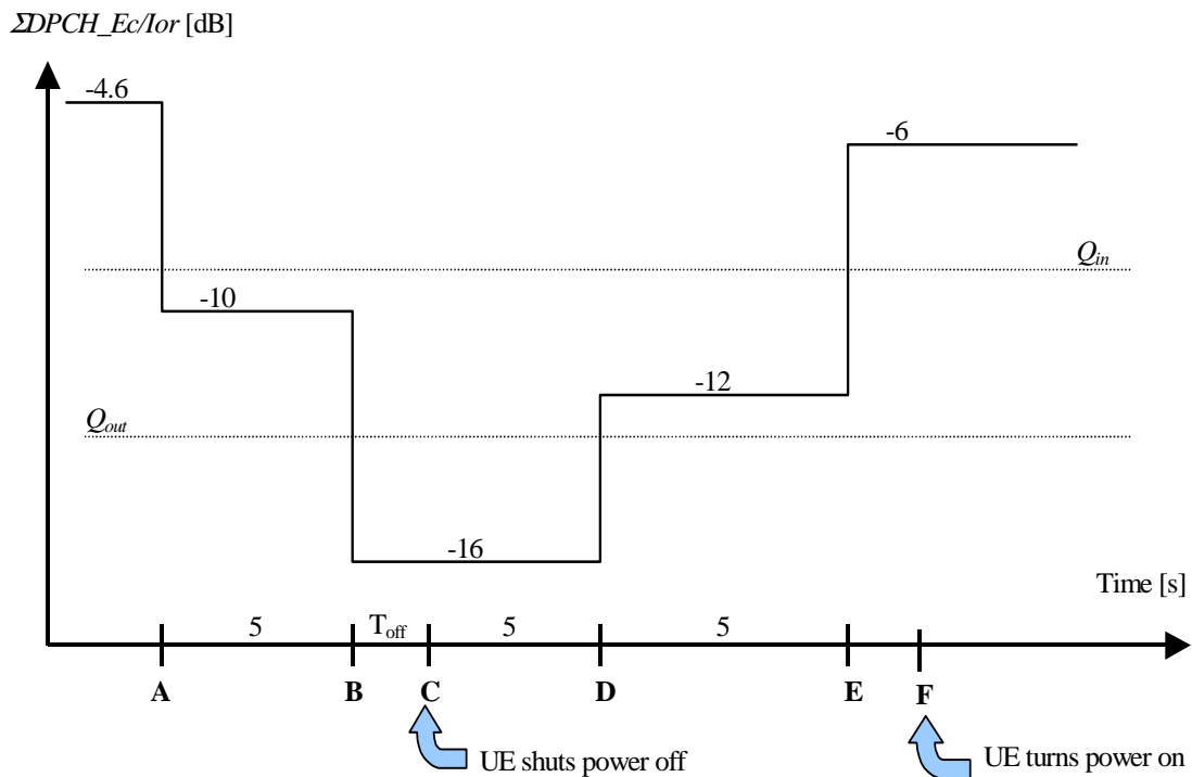
Figure 5.4.5.1: Test case for out-of-synch handling in the UE.
