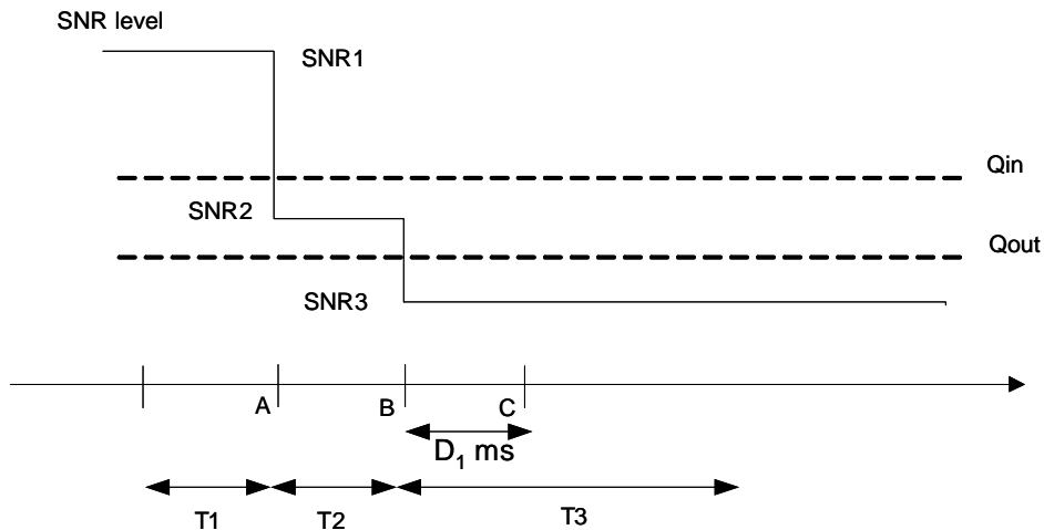
Figure A.7.3.5.1-5 SNR variation for out-of-sync testing in DRX
