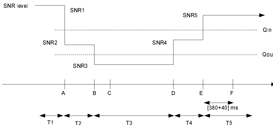
Figure A.7.3.2.1-3 SNR variation for in-sync testing
