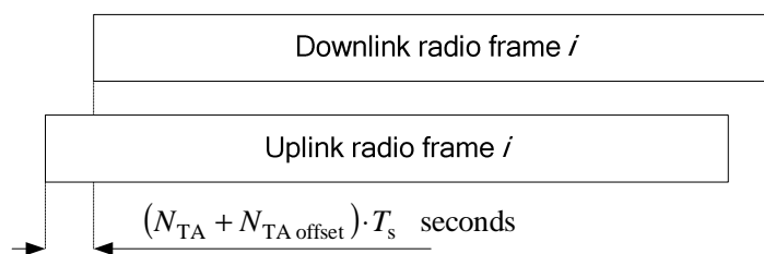
Figure 8.1-1: Uplink-downlink timing relation.
