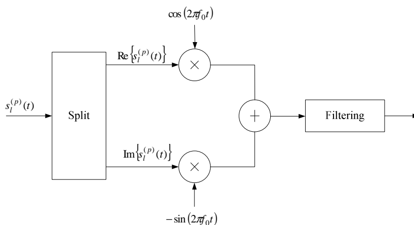
Figure 6.13-1: Downlink modulation.
