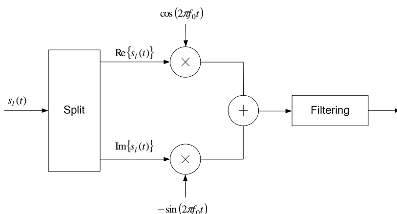
Figure 5.8-1: Uplink modulation.
