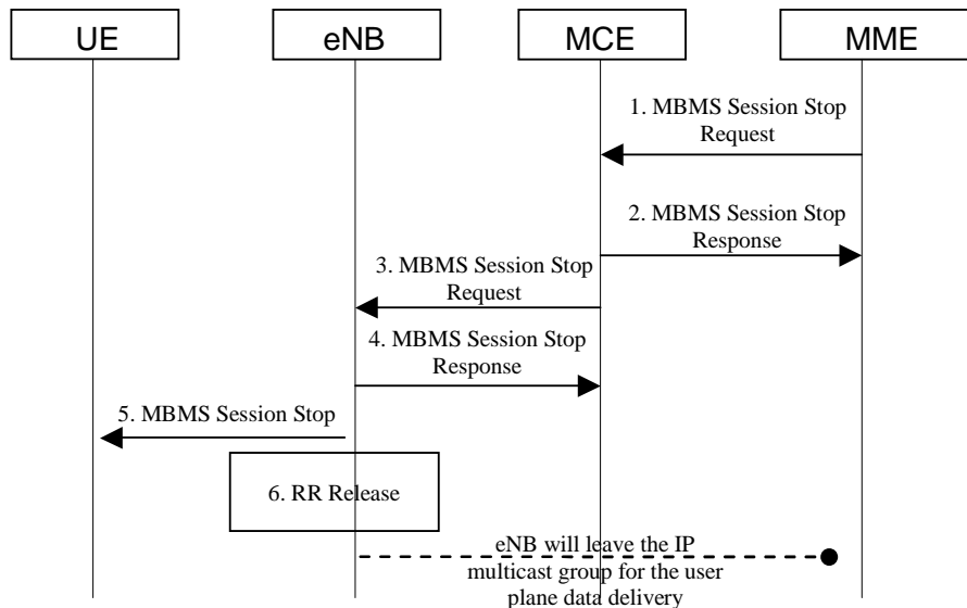
Figure 15.7.1.2-1. Session Stop procedure
