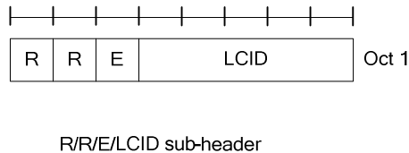
Figure 6.1.6-2: R/R/E/LCID MAC subheader
