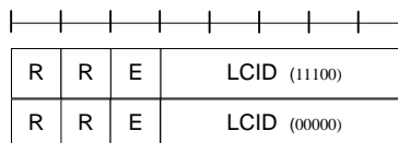
Case 2: MAC subheader for MAC control element + MAC subheader for MAC SDU (CCCH)
