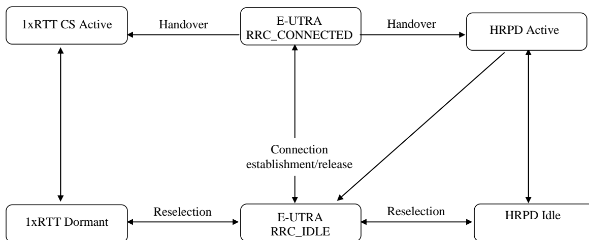
Figure 4.2.1-2: Mobility procedures between E-UTRAN and CDMA2000
