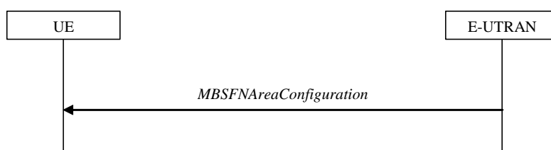
Figure 5.8.2.1-1: MCCH information acquisition, normal
