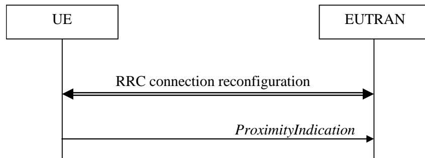
Figure 5.3.14.1-1: Proximity indication
