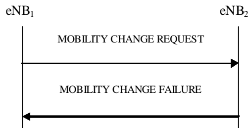
Figure 8.3.8.3-1: Mobility Settings Change, unsuccessful operation
