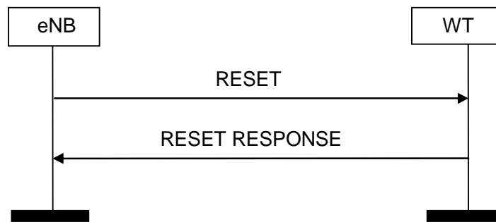
Figure 8.7.2-1: Reset, eNB-initiated. Successful operation.
