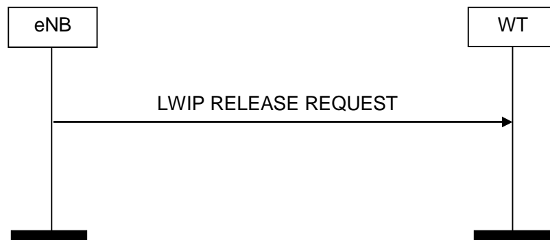
Figure 8.16.2-1: eNB initiated LWIP Release, successful operation
