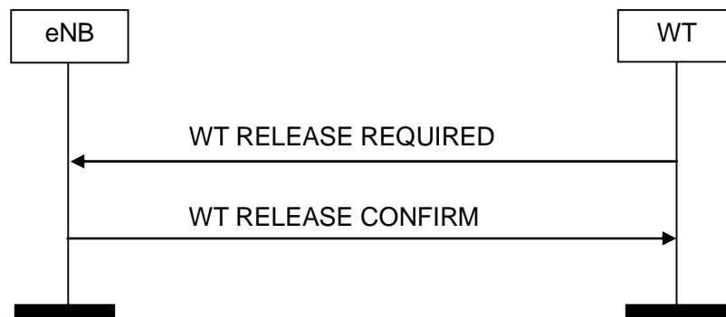
Figure 8.12.2-1: WT initiated WT Release, successful operation
