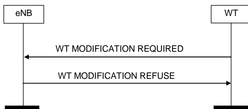
Figure 8.10.3-1: WT initiated WT Modification, unsuccessful operation
