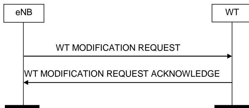
Figure 8.9.2-1: eNB initiated WT Modification, successful operation
