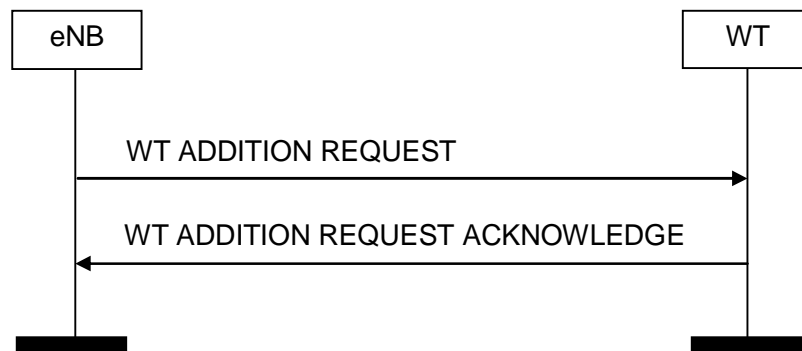
Figure 8.8.2-1: WT Addition Preparation, successful operation
