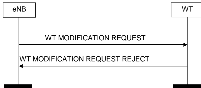
Figure 8.9.3-1: eNB initiated WT Modification, unsuccessful operation
