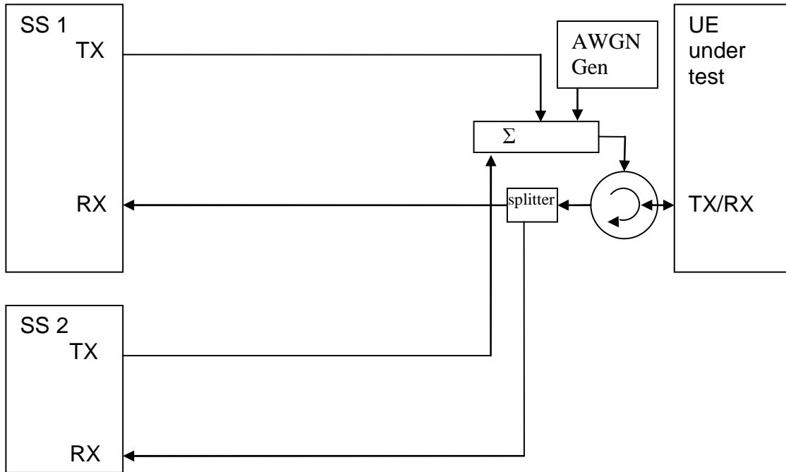
Figure A.12: Connection for 2 cells with static propagation
