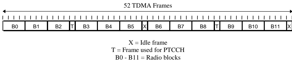
Figure 2: Multiframe structure for PDCH
