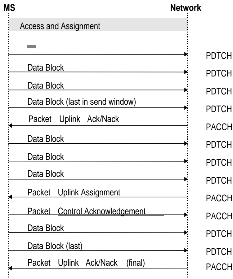
Figure 25: An example of dynamic allocation uplink data transfer
