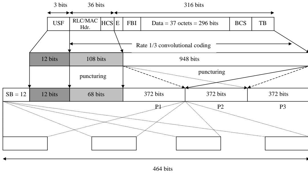
Figure 16: Coding and puncturing for MCS-3; rate 0.80 GMSK, one RLC block per 20 ms
