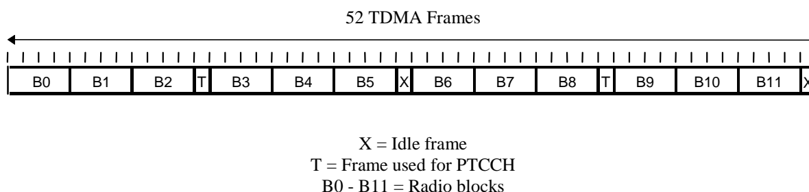
Figure 2: Multiframe structure for PDCH
