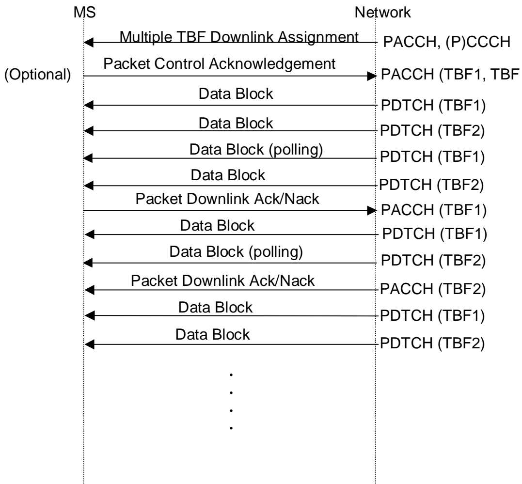
Figure 28: An example of downlink data transfer with two TBFs
