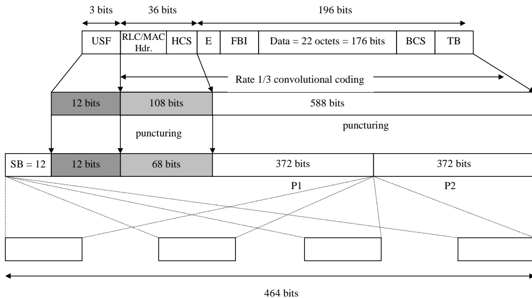
Figure 18: Coding and puncturing for MCS-1; rate 0.53 GMSK, one RLC block per radio block
