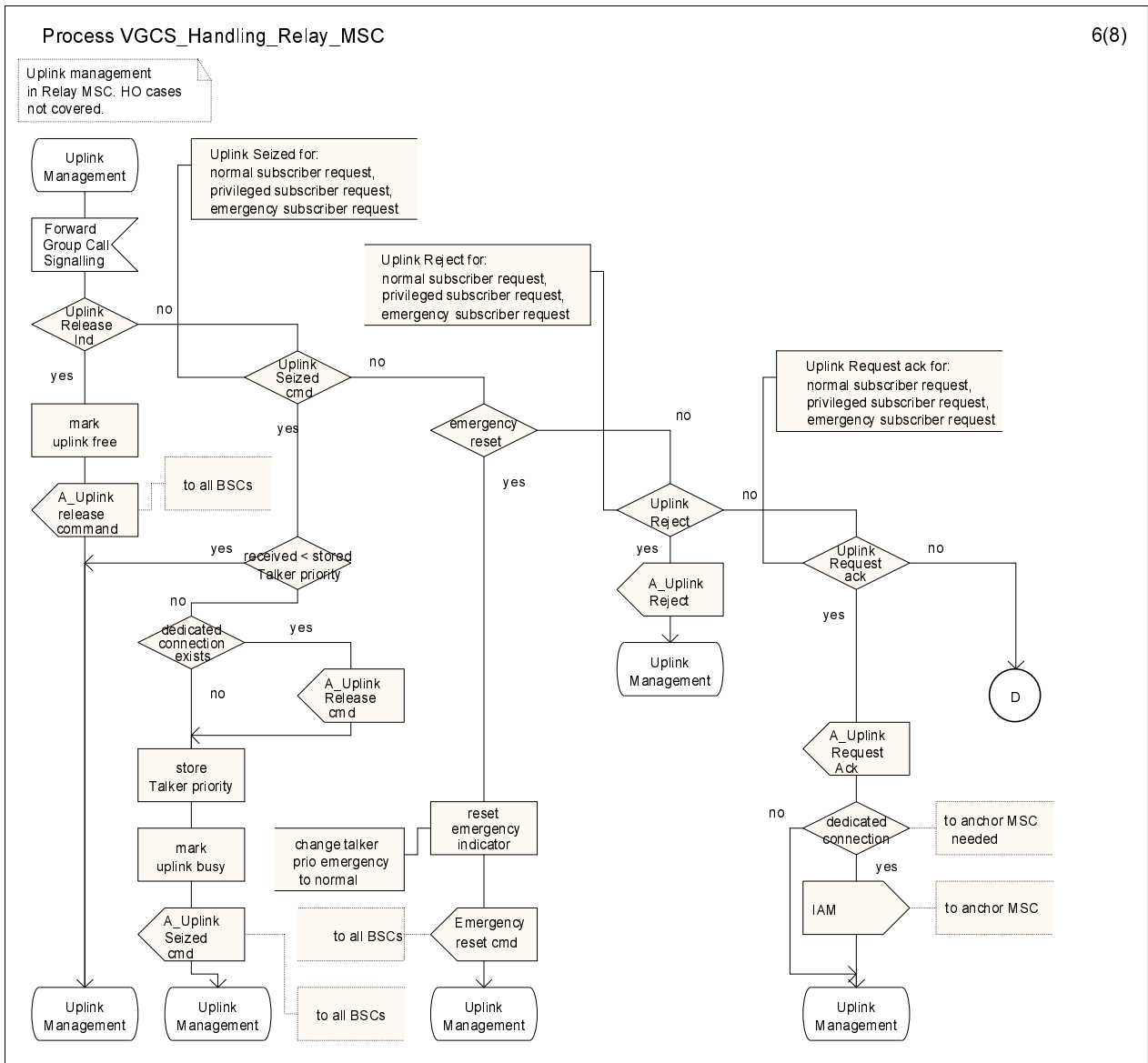
Figure 10: The VGCS handling process in the relay MSC (sheet 6 of 8)
