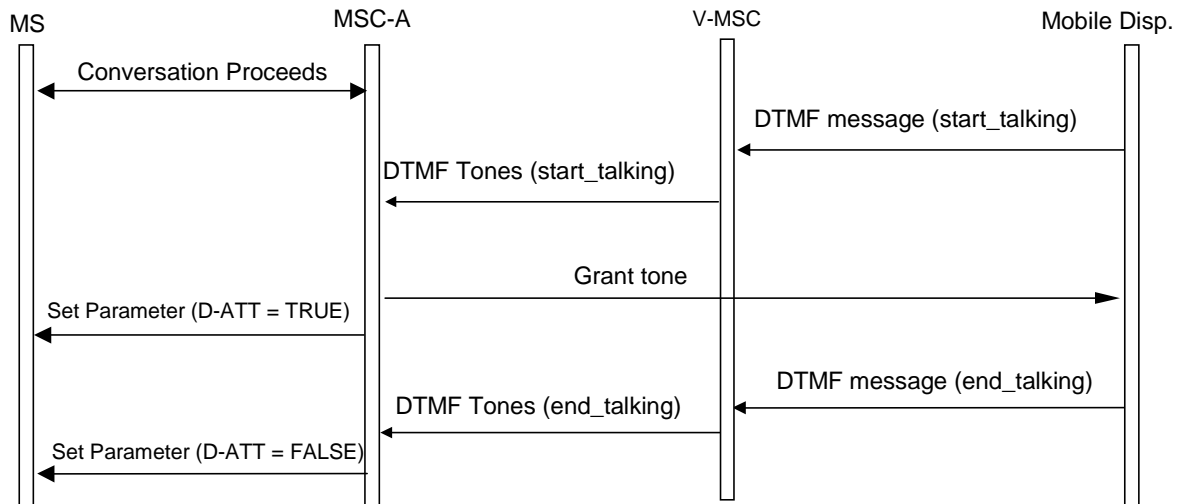
Figure 5c: Signalling information required when the talker is attached to the Anchor MSC and a mobile dispatcher who is roaming in a non-Anchor MSC area wishes to speak
