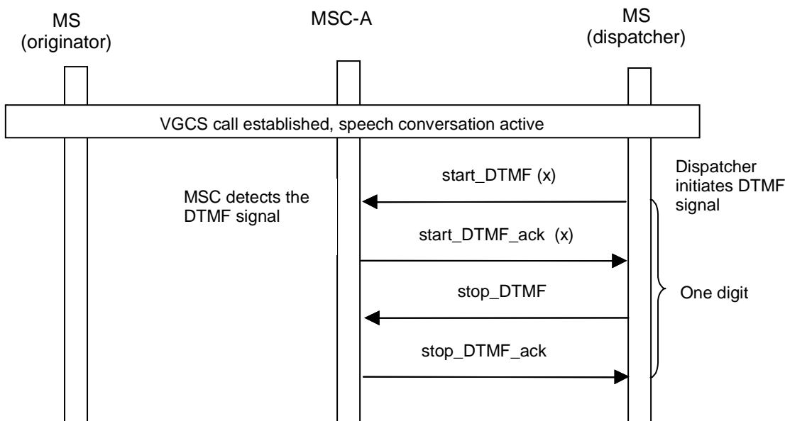
Figure 7b: Signalling required for communication of DTMF digit entry by an entitled mobile dispatcher, if the mobile dispatcher is controlled by the anchor MSC of the group call.
