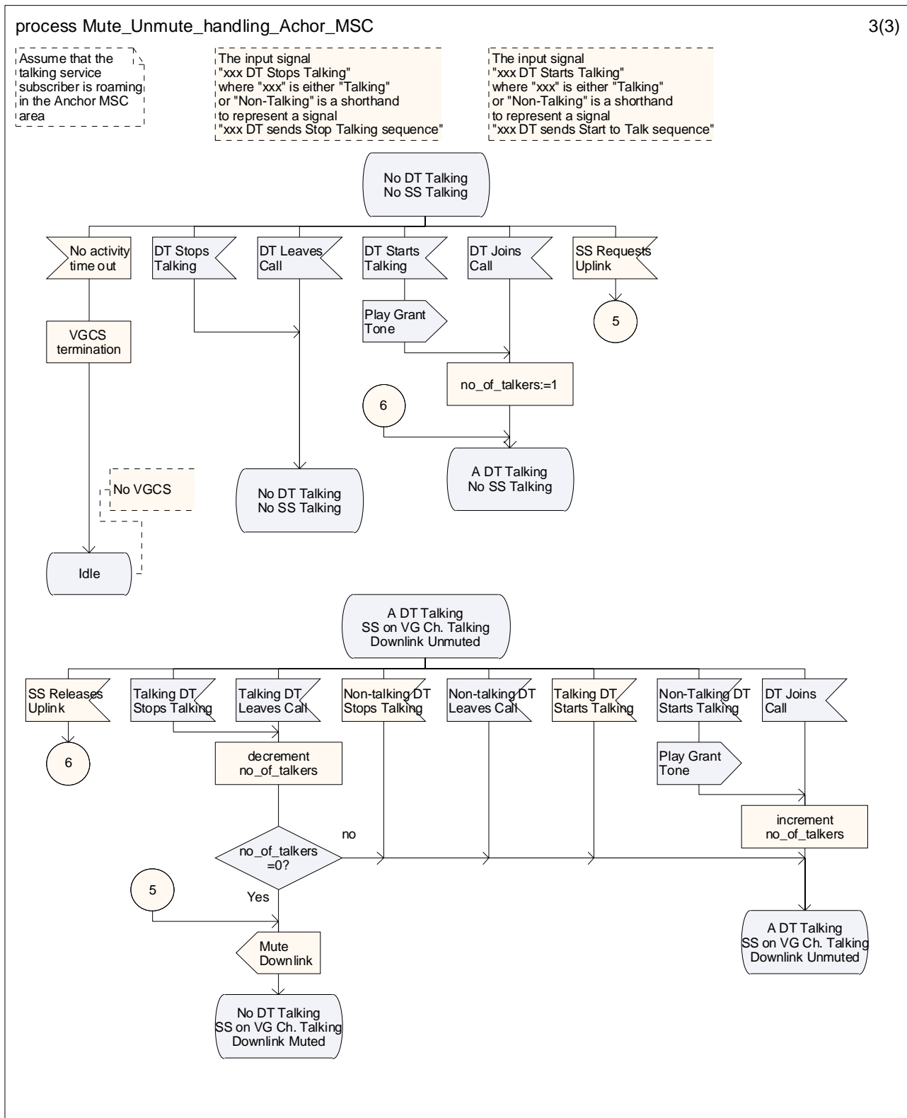
Figure 1a: Handling of Mute/Unmute Requests in Anchor MSC (Sheet 3 of 3)
