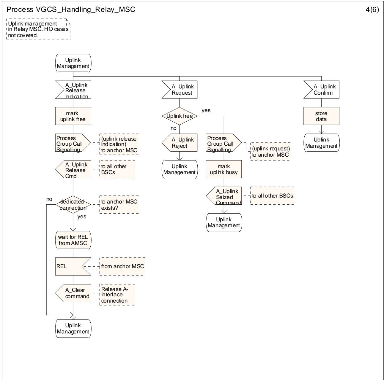
Figure 10: The VGCS handling process in the relay MSC (sheet 4 of 6)
