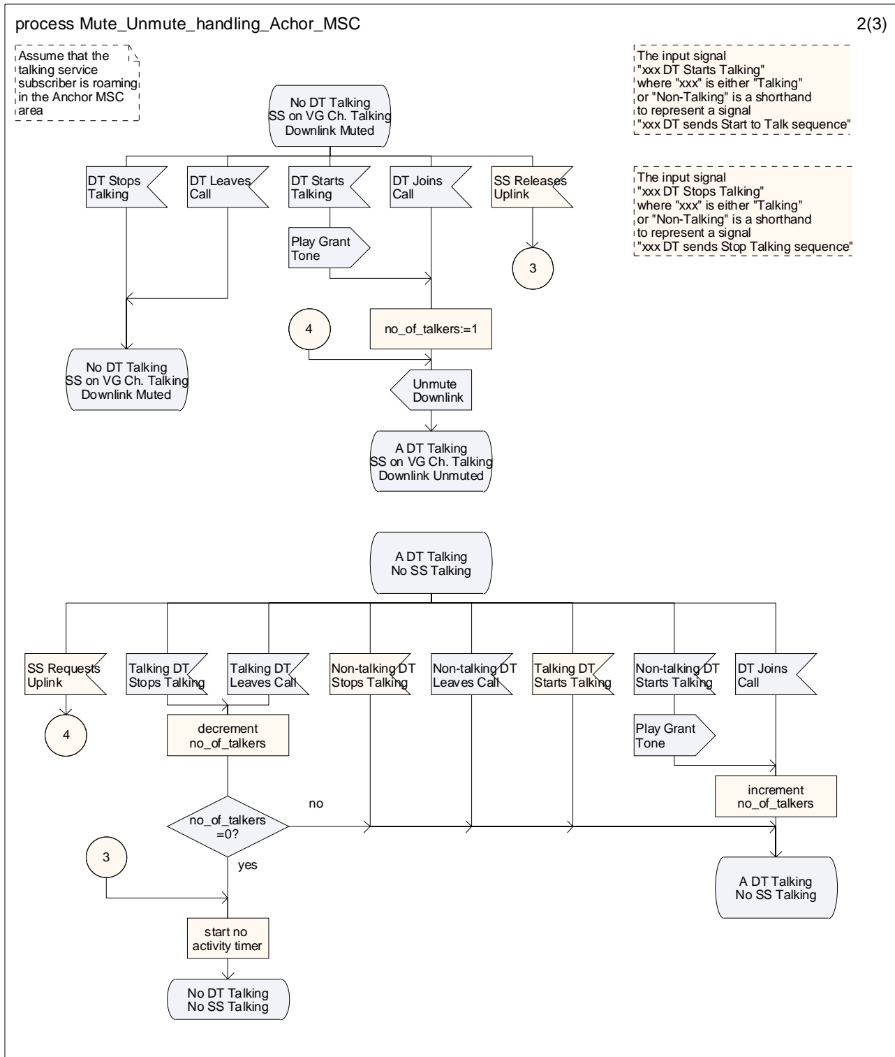
Figure 1a: Handling of Mute/Unmute Requests in Anchor MSC (Sheet 2 of 3)
