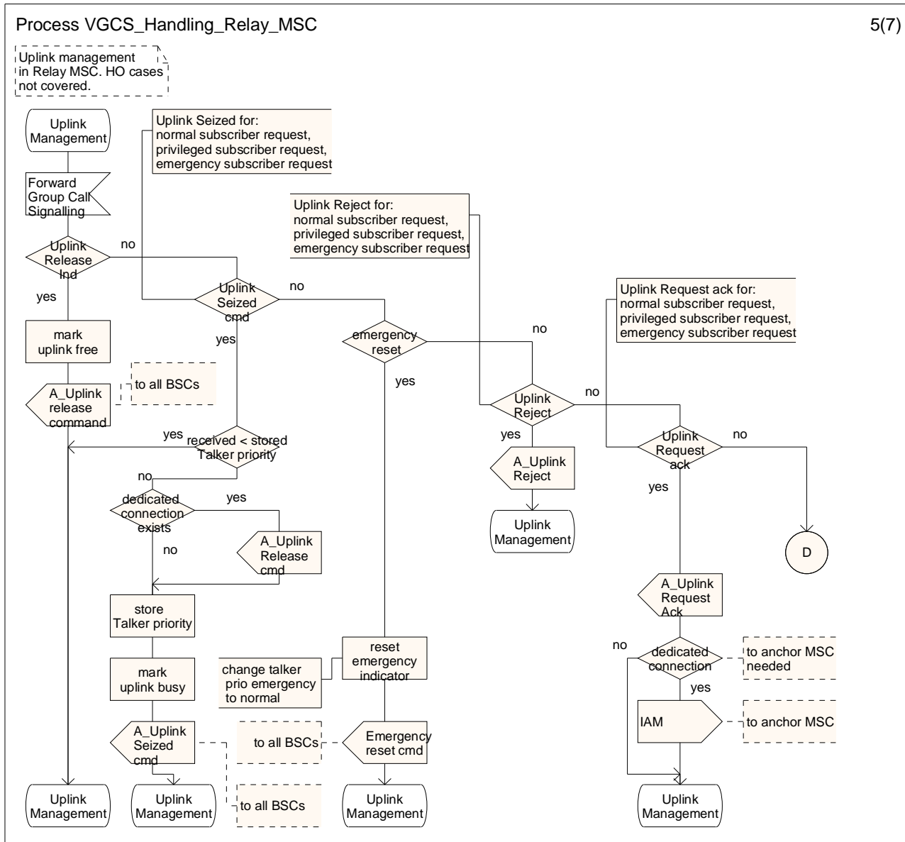
Figure 10: The VGCS handling process in the relay MSC (sheet 5 of 7)
