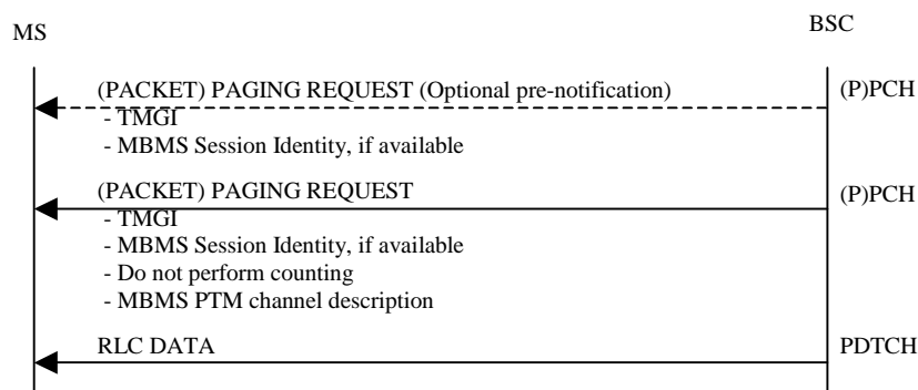
FIGURE 6.1.1.3.c: PTM Bearer established
