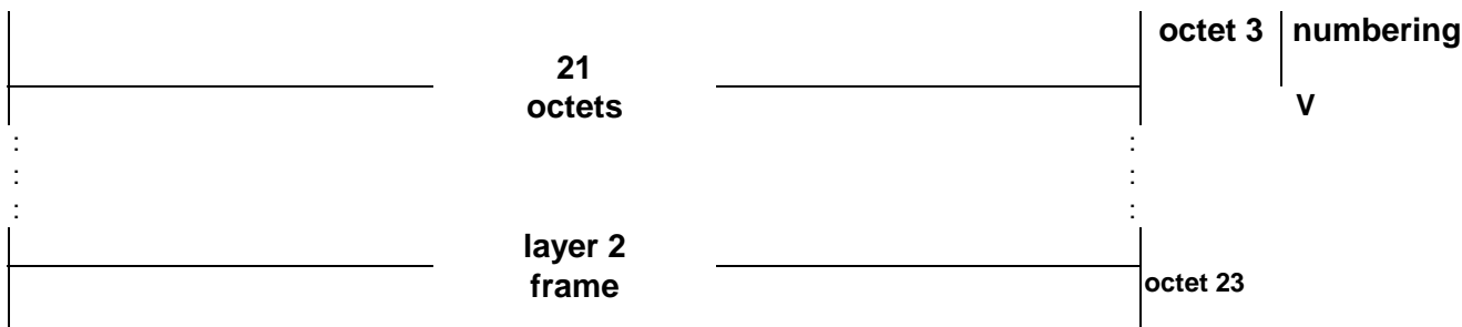
Figure 7.1.1: SACCH downlink block format for MS operating in A/Gb mode
