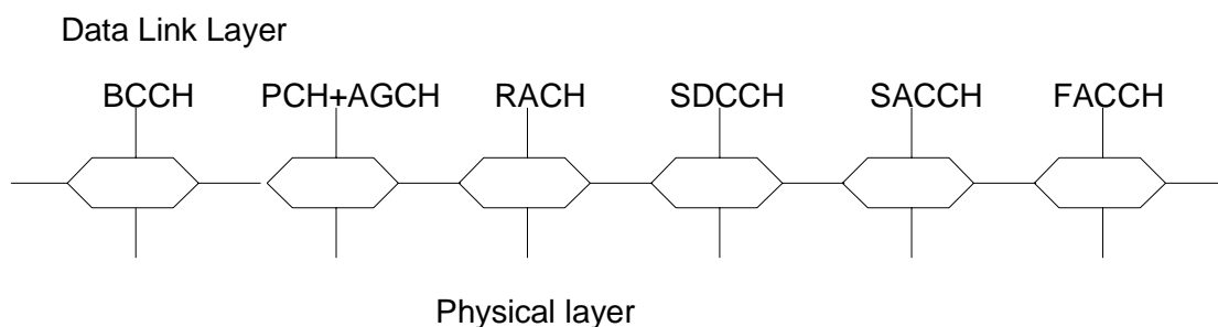
Figure 3.a.b: SAPs between the physical layer and the data link layer in the MS
