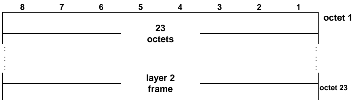
Figure 7.3: FACCH/SDCCH/BCCH/CCCH/CBCH downlink block format
