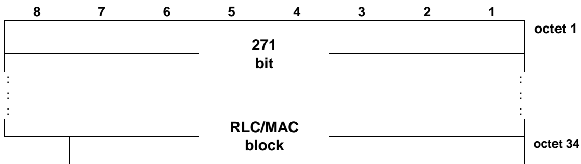
Figure 7.6.2: PDTCH block type 2 (CS-2) format
