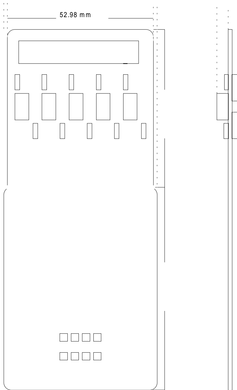
Figure 3: Dimensions of full size paddle
