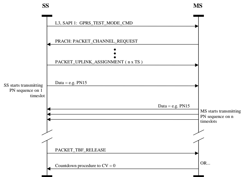
Figure 5.4.3: PN Sequence Definition
