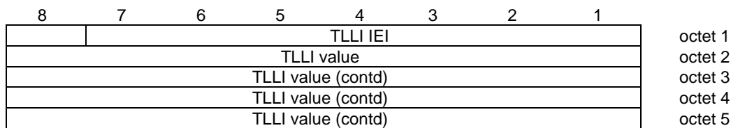
Figure 10.5.2.41a.1: TLLI information element
