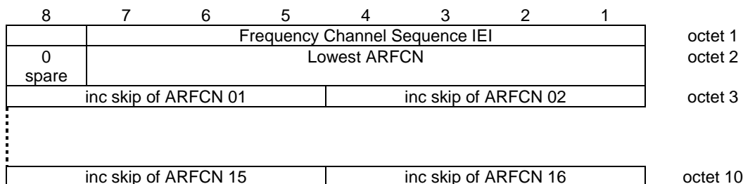
Figure 10.5.2.12.1/3GPP TS 44.018: Frequency Channel Sequence information element
