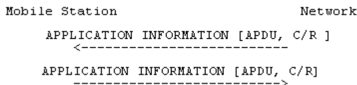
Figure 3.4.21.3.4.1/3GPP TS 44.018: Application Information Transfer without segmentation
