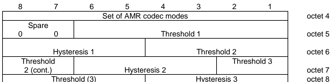
Figure 10.5.2.21aa.5/3GPP TS 44.018: Parameters for multirate speech field for the MR version 1 when a set of four modes is chosen
