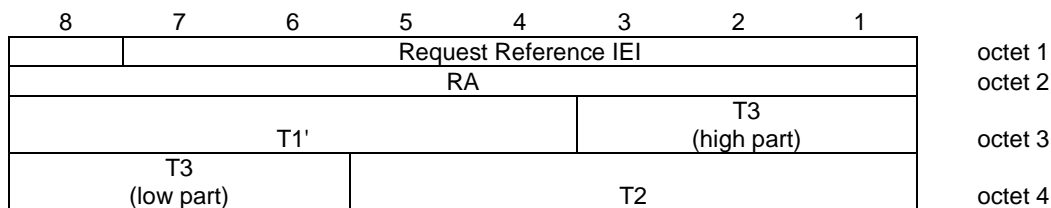
Figure 10.5.2.30.1/3GPP TS 44.018: Request Reference information element
