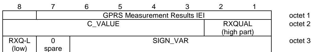
Figure 10.5.2.20a.1/3GPP TS 44.018: GPRS Measurement Results information element
