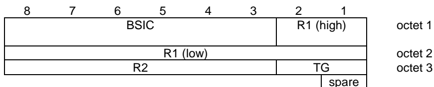
Figure 9.1.30b.1/3GPP TS 44.018: COMPACT Frame synchronization information element
