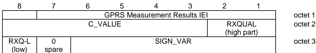
Figure 10.5.2.20a.1: GPRS Measurement Results information element
