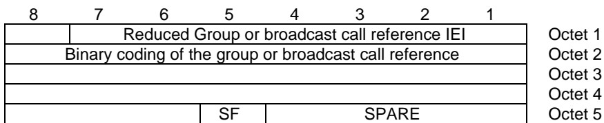
Figure 10.5.2.63.1 Reduced Group or Broadcast Call Reference
