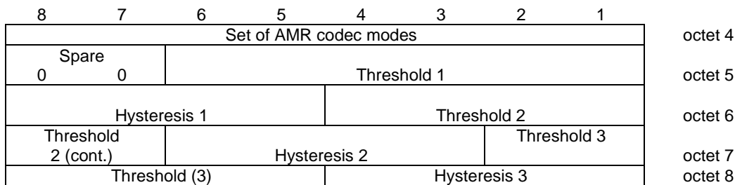
Figure 10.5.21aa.5: Parameters for multirate speech field for the Multirate speech versions 1 & 2 when a set of four modes is chosen
