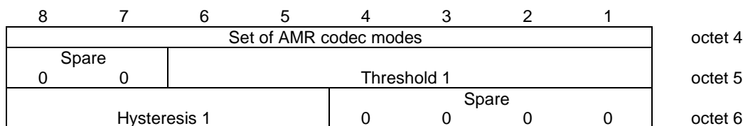
Figure 10.5.2.21aa.3/3GPP TS 04: Parameters for multirate speech field for the Multirate speech versions 1 & 2 when a set with two codec modes is chosen
