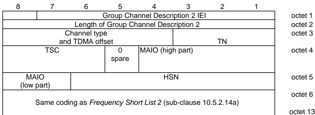
Figure 10.5.2.14f.1: Group Channel Description 2 information element
