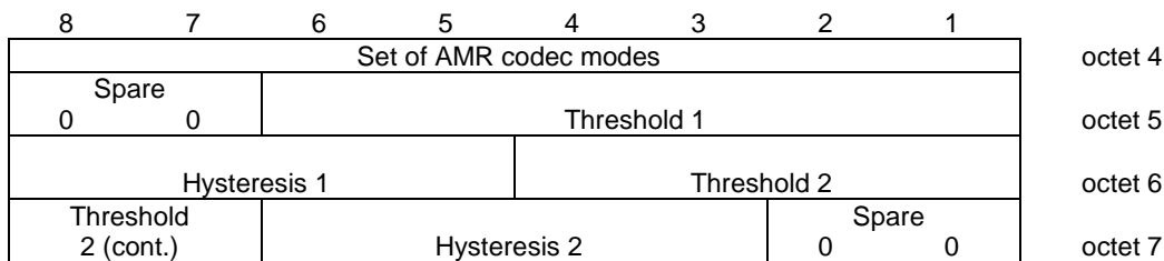
Figure 10.5.21aa.4: Parameters for multirate speech field for the Multirate speech versions 1 & 2 when a set of three codec modes is chosen
