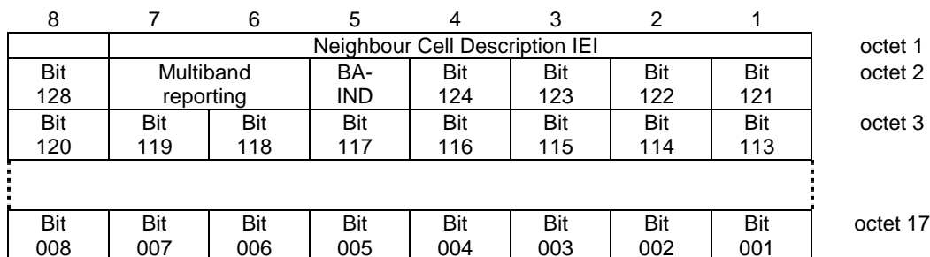
Figure 10.5.2.22a.1: Neighbour Cell Description 2 information element
