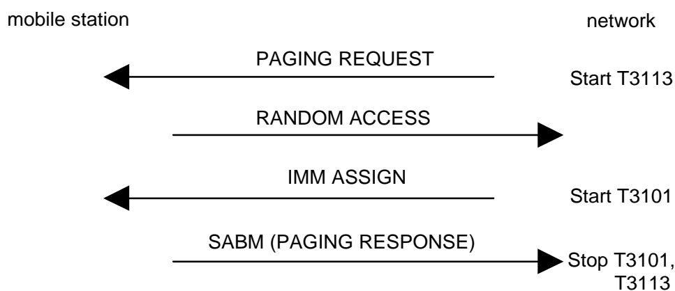
Figure 3.3.2.3.1: Paging sequence
