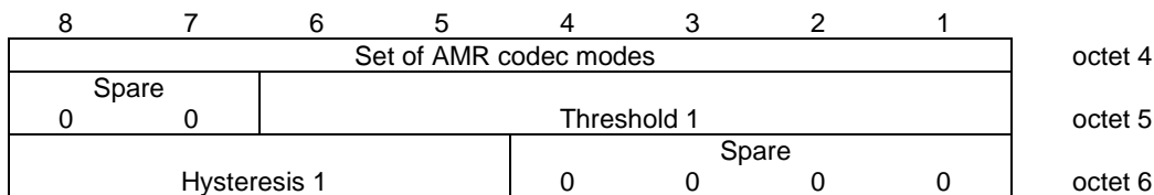
Figure 10.5.2.21aa.3: Parameters for multirate speech field for the Multirate speech versions 1 & 2 when a set with two codec modes is chosen
