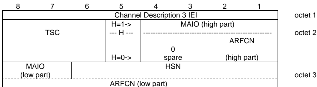
Figure 10.5.2.5c.1: Channel Description information element
