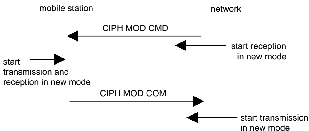
Figure 3.4.7.2.1: Ciphering mode setting sequence
