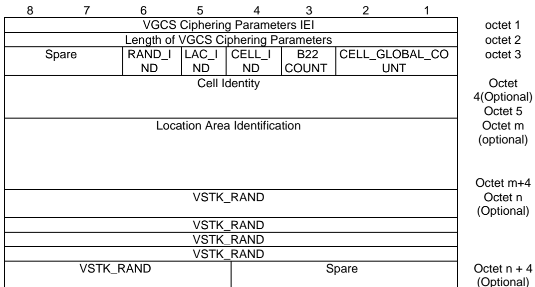
Figure 10.5.2.42b.1: VGCS Ciphering Parameters Information Element
