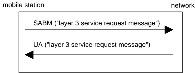
Figure 3.1.5.1: Service request and contention resolution
