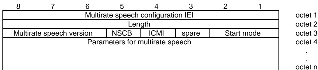
Figure 10.5.2.21aa.1: MultiRate configuration information element
