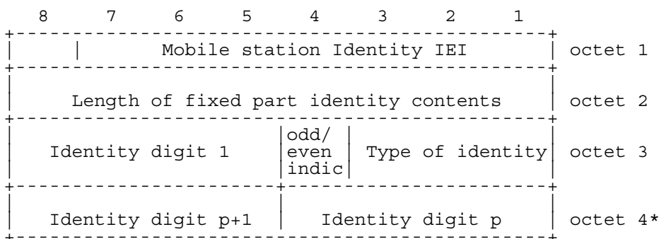
Figure 10.5/GSM 04.xx: Mobile station Identity information element
