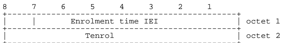
Figure 10.5/GSM 04.xx: Enrolment time information element
