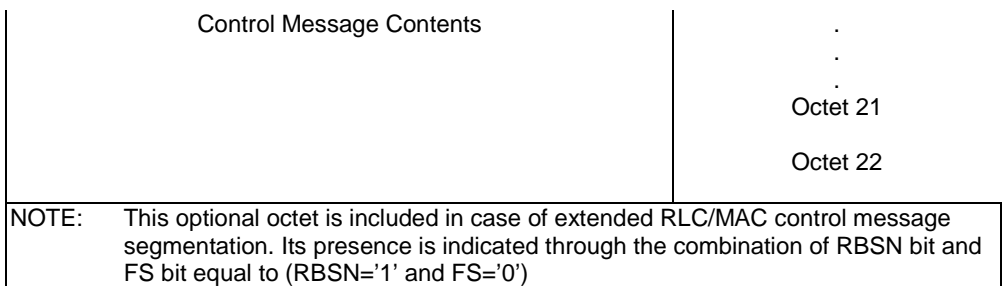
Figure 10.3.1.1: Downlink RLC/MAC control block together with its MAC header
