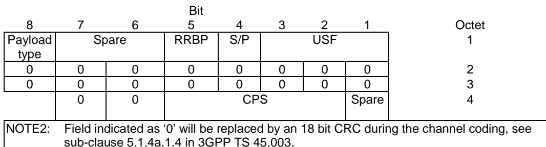
Figure 10.3a.3.3.3: Downlink RLC/MAC control block header for MCS-0.
