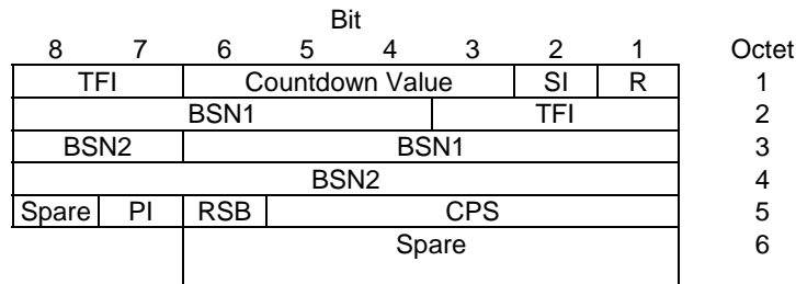
Figure 10.3a.4.1.1: EGPRS uplink RLC data block header (FANR not activated) for MCS-7, MCS-8 and MCS-9.
