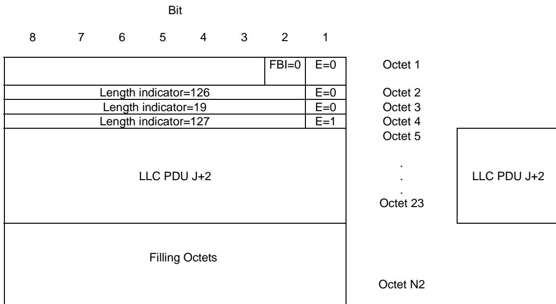
Figure B.11: Example for the case when the LLC PDU J+1 ends in the previous RLC data block and the start of the next LLC PDU J+2 is in the next RLC data block which is indicated using LI=126 as the first LI in that RLC data block.
