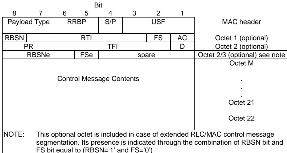
Figure 10.3.1.1.1: Downlink RLC/MAC control block together with its MAC header
