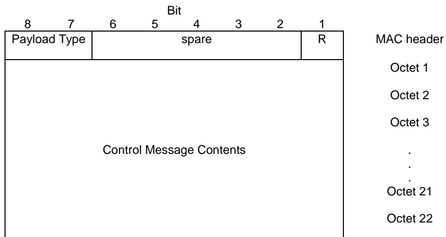
Figure 10.3.2.1: Uplink RLC/MAC control block together with its MAC header
