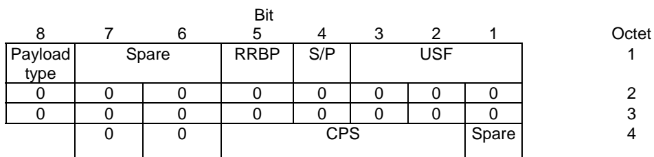
Figure 10.3a.3.3.3: Downlink RLC/MAC control block header for MCS-0.
