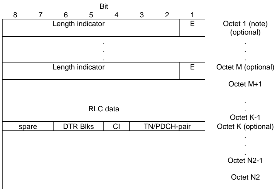
Figure 10.3a.1.1.1: EGPRS downlink RLC data block
