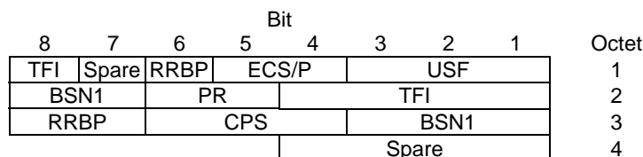
Figure 10.3a.3.2.5: EC-GSM-IoT downlink RLC data block header for MCS-5 and MCS-6
