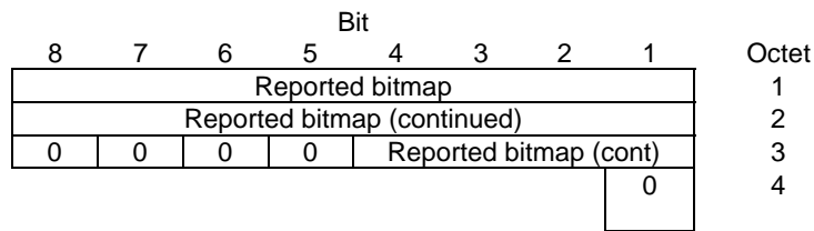
Figure 10.3a.6.1: Piggy-backed Ack/Nack field (Time-based)
