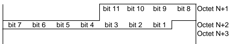
Figure 11.1: Field mapping within RLC/MAC messages
