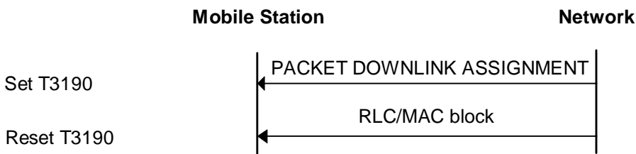
Figure C.2: TBF establishment initiated by the network
