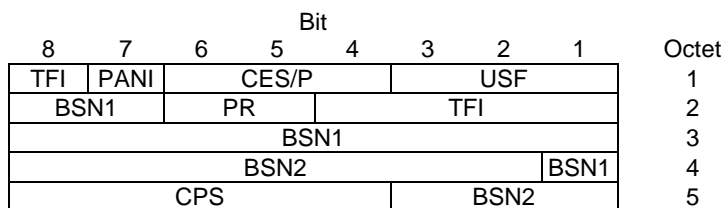
Figure 10.3a.3.1.2: EGPRS downlink RLC data block header (FANR activated) for MCS-7, MCS-8 and MCS-9.
