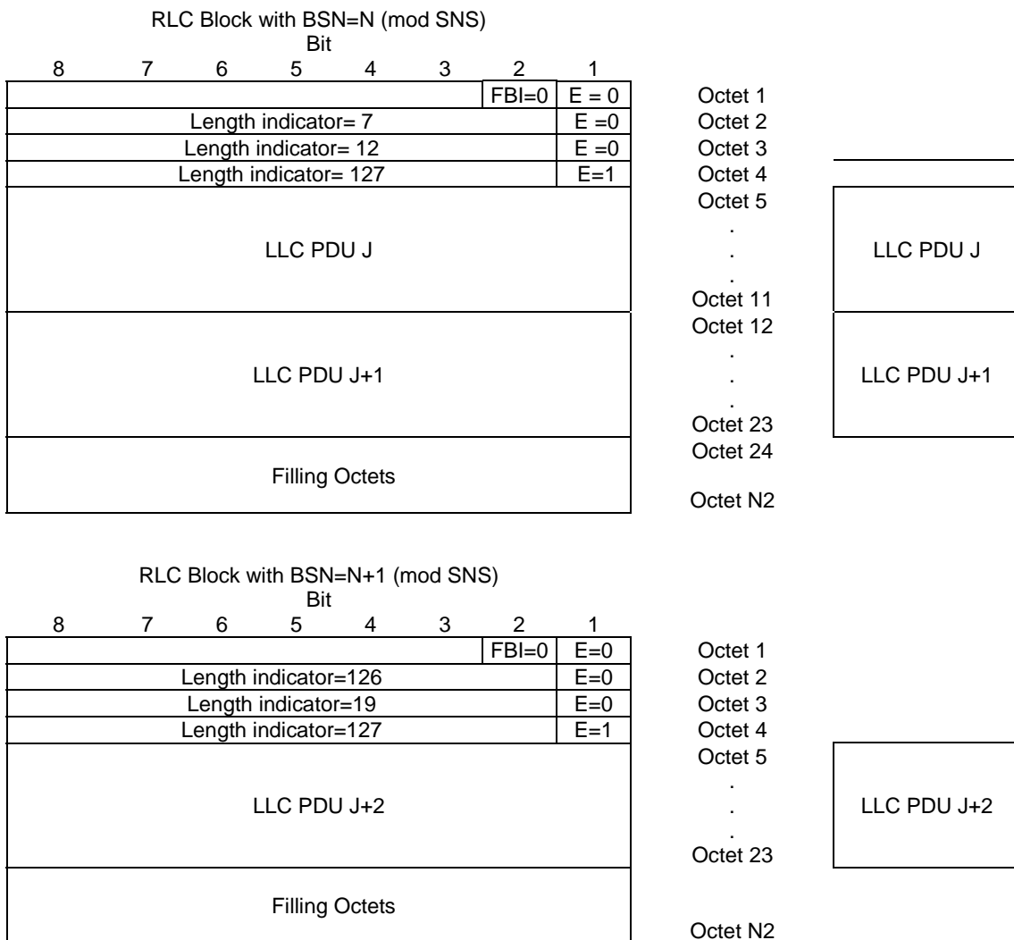
Figure B.11: Example for the case when the LLC PDU J+1 ends in the previous RLC data block and the start of the next LLC PDU J+2 is in the next RLC data block which is indicated using LI=126 as the first LI in that RLC data block.
