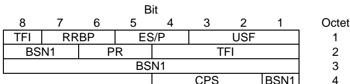
Figure 10.3a.3.2.1: EGPRS downlink RLC data block header (FANR not activated) for MCS-5 and MCS-6
