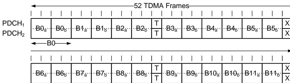
Figure 2a3: 52- multiframe for a PDCH-pair in RTTI configuration.
